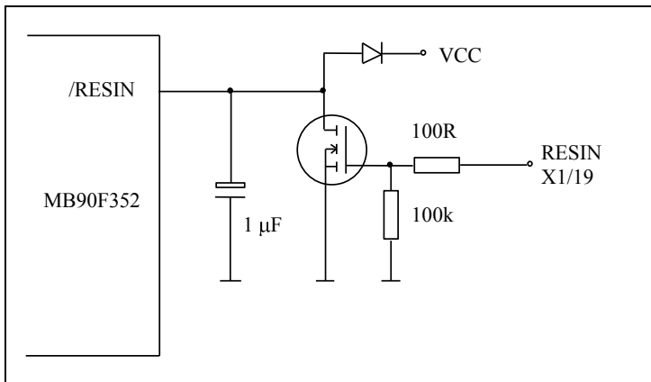
Figure 4: structure of /RESIN Line
