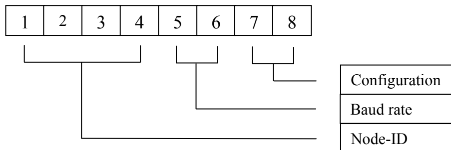
Figure 2: DIP-switch Pinout and Functions
