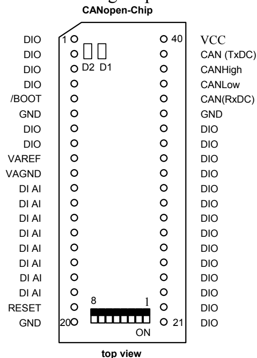
Figure 1: Pin Layout
