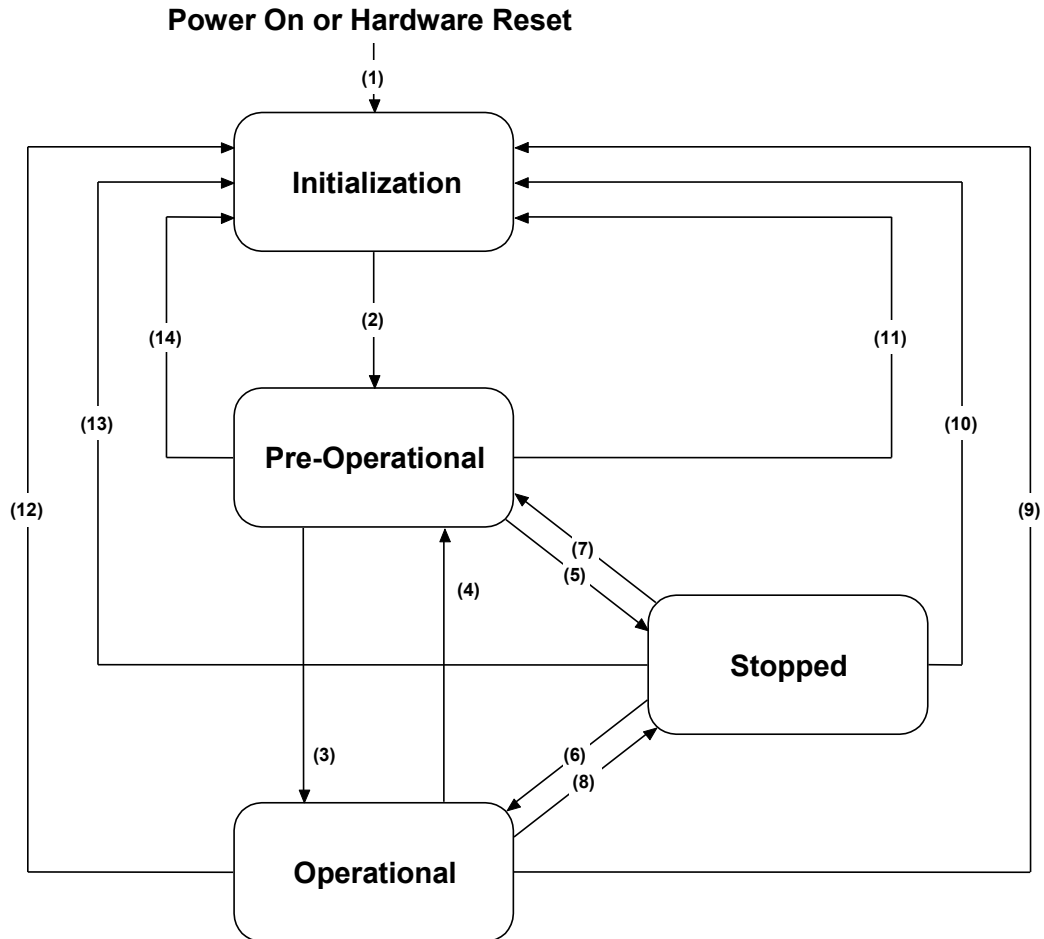
Figure 5: State Diagram of a CANopen Device
