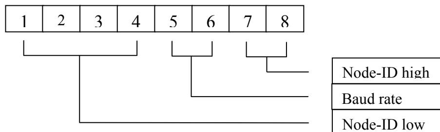
Figure 2: DIP-switch Pinout and Functions
