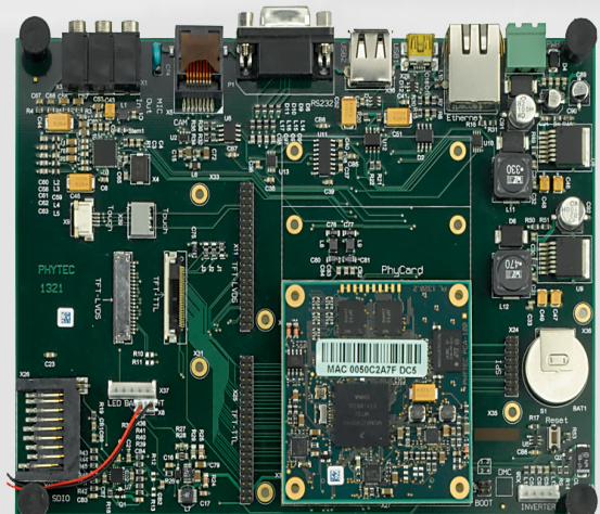
phyCARD-S on phyBASE The phyBASE accommodates the varying dimensions of all phyCARDS.
